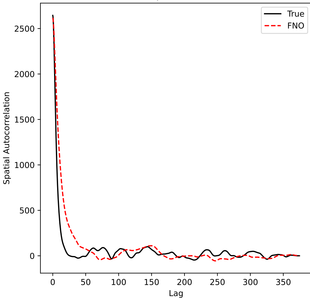
Autocorrelation Comparison with MSE = 2.1 \times 10^4
