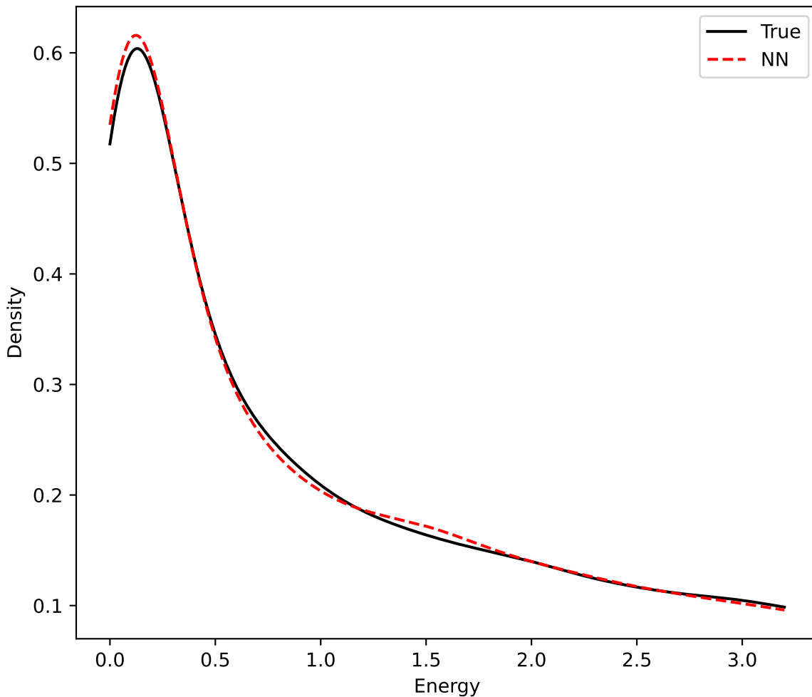
TKE Density Comparison with KS: 0.011, p-value: 2.9e-05
